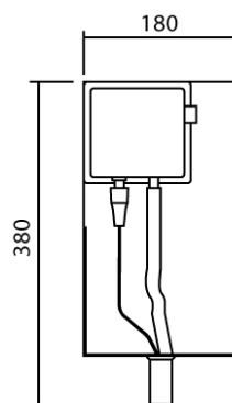
MODEL : MBM-103 (mm.)
